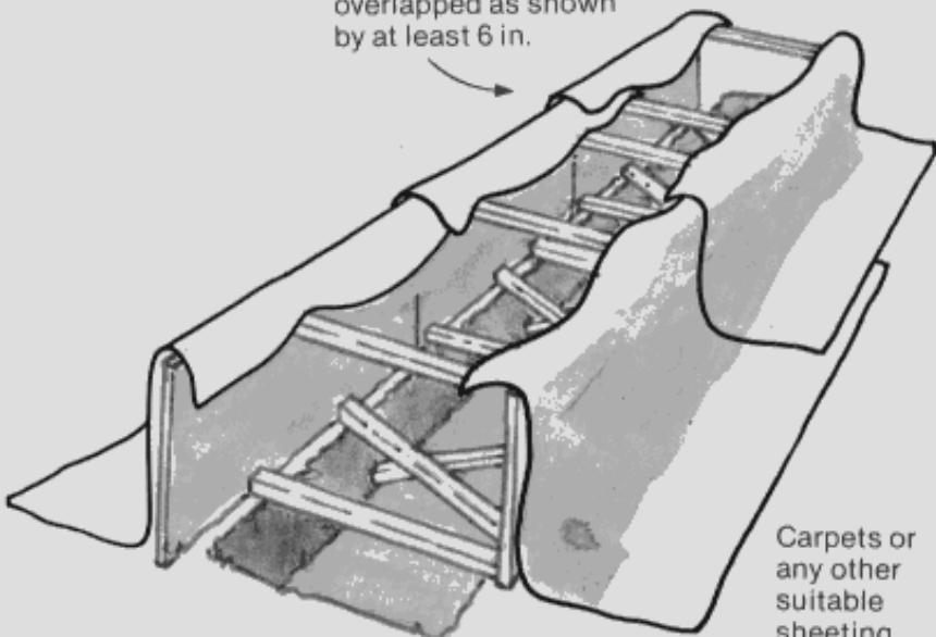
Fig 7 Position sheeting material
