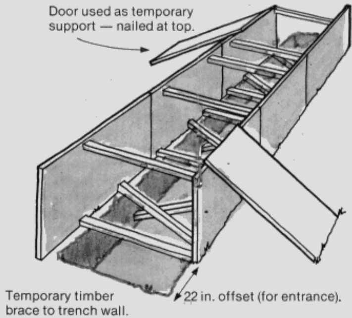
Fig 6 Construct temporary walls
