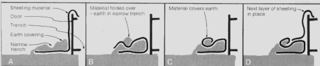
Fig 8 - Construction of earth rolls
