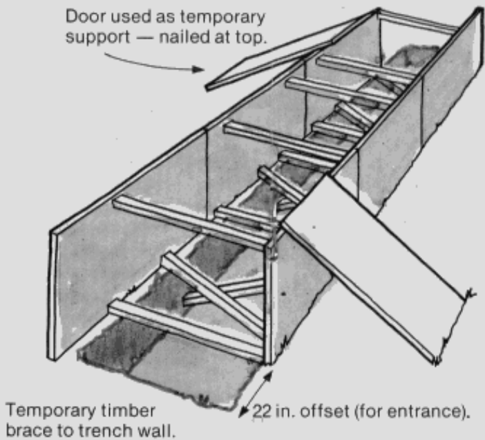
Fig 6 Construct temporary walls
